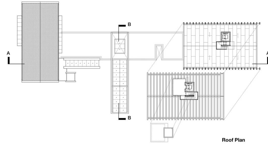
Roof Plan
