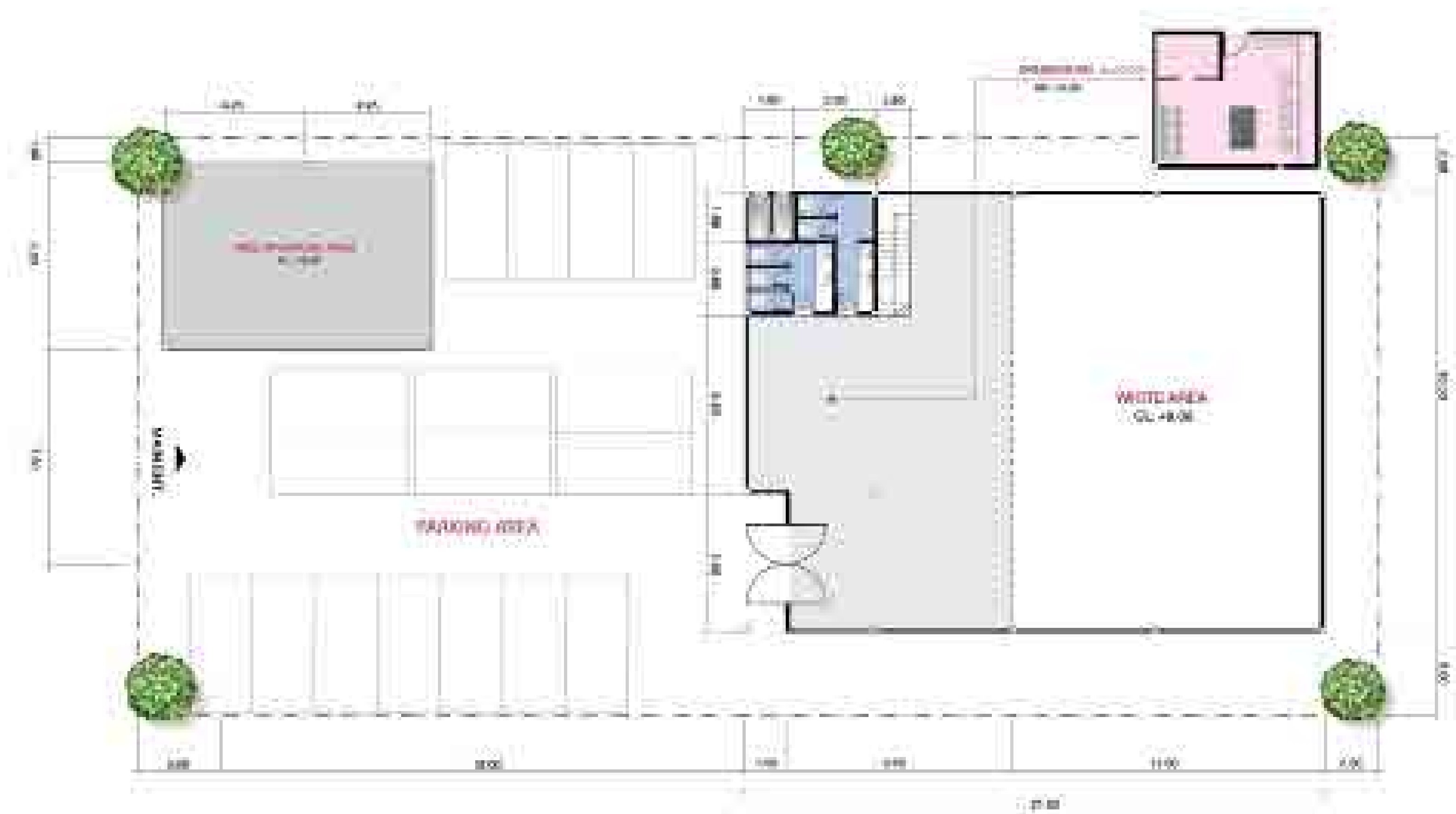
FLOOR PLAN STUDIO RAMNTRA
